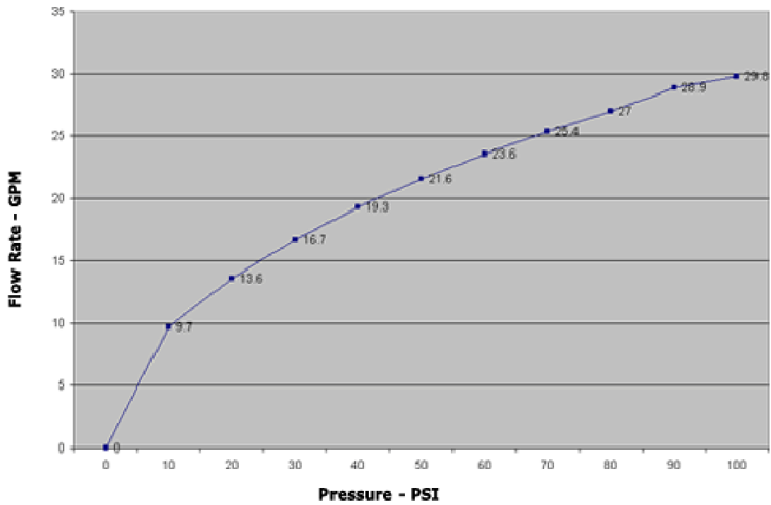
Hudson Valve 1/2" Flow Rate Chart
